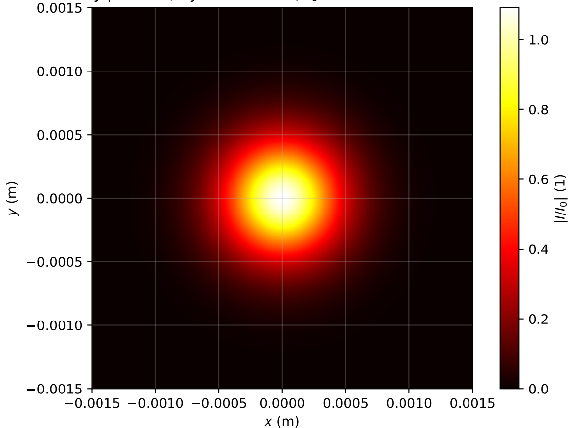
Intensity profile I(x, y, z = 0.637m)/I_0 , Pin=0.6Pcr, artificial time
